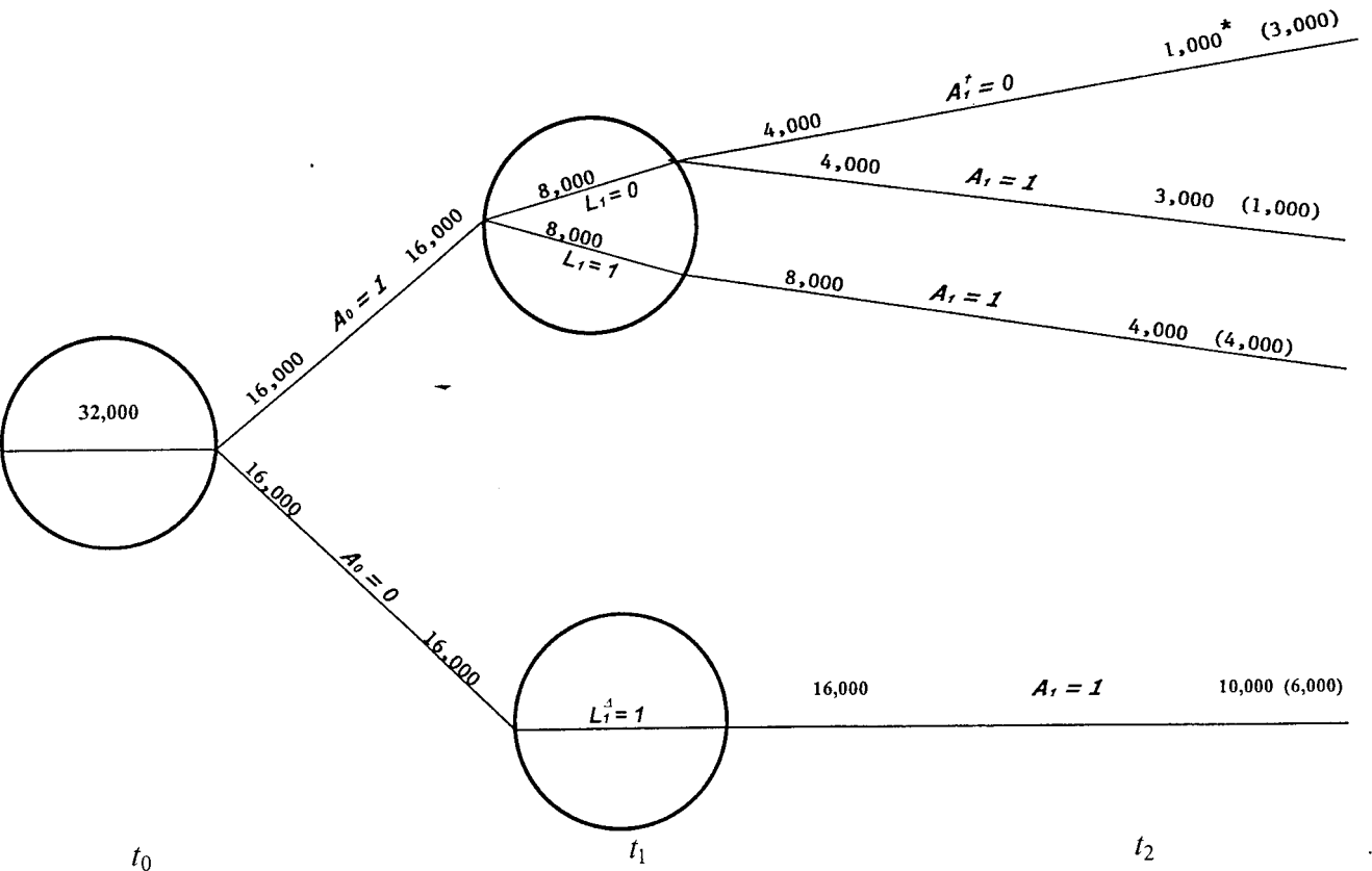
FIG. 10. Data from a hypothetical study: (*) survivors ( Y = 1 ) at t_2 [Deaths ( Y = 0 ) at t_2 in parentheses]; ( \dagger ) A_k measured just after time t_k , k = 0, 1 ; ( \ddagger ) L_1 measured at time t_1 .
